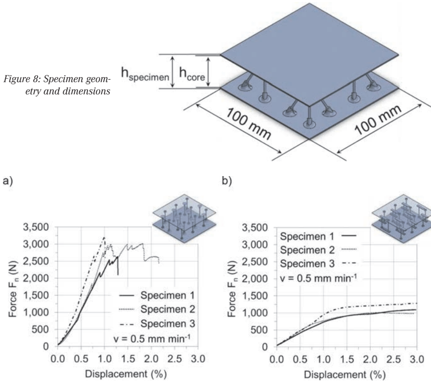
Figure 9: Compression tests with a hexagonal lattice core structure nominal force vs. displacement diagram, a) DIF, b) CLF
