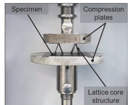
Figure 7: Experimental setup of compression test according to ASTM C365 C365/M
