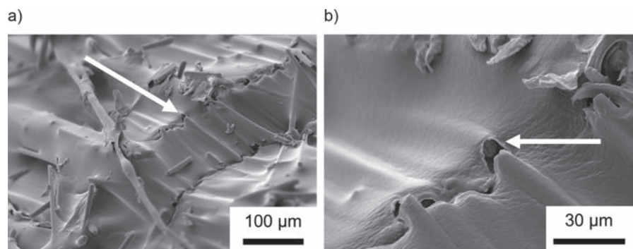
Figure 11: SEM recording of failure in the middle of the CFRP-rod, a) kink band, b) detail of kink band with perpendicular carbon fiber failure surface within PA12 matrix
