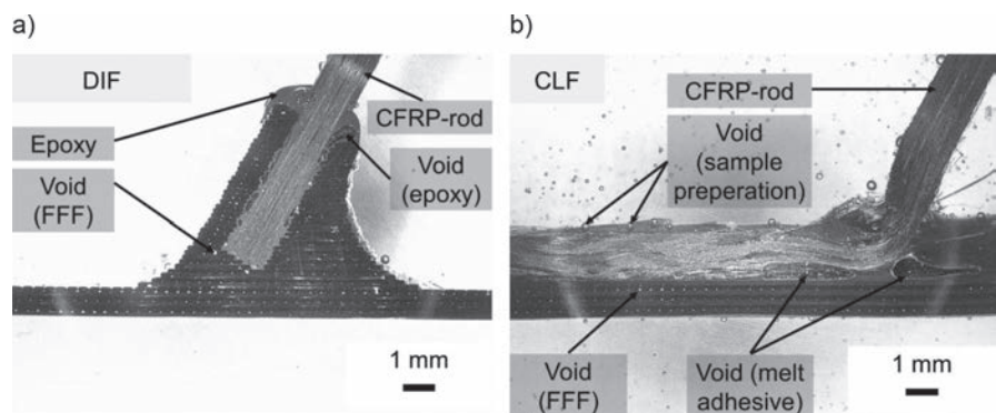
Figure 12: Optical microscope of cross sections, a) plug-in connector (DIF), b) interface (CLF)
