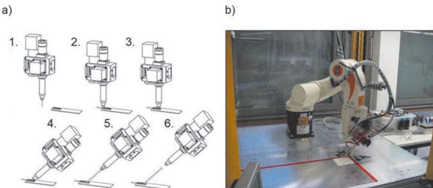
Figure 4: Manufacturing of CFRP-rod (CLF), a) motion cycle of CLF-application head, b) production cell with six-axis robot und CLF-application head
