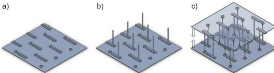
Figure 2: Scheme for continuous lattice fabrication (CLF) process steps, a) individual top layers (FFF), b) manufacturing of lattice core structure, c) manual assembly
