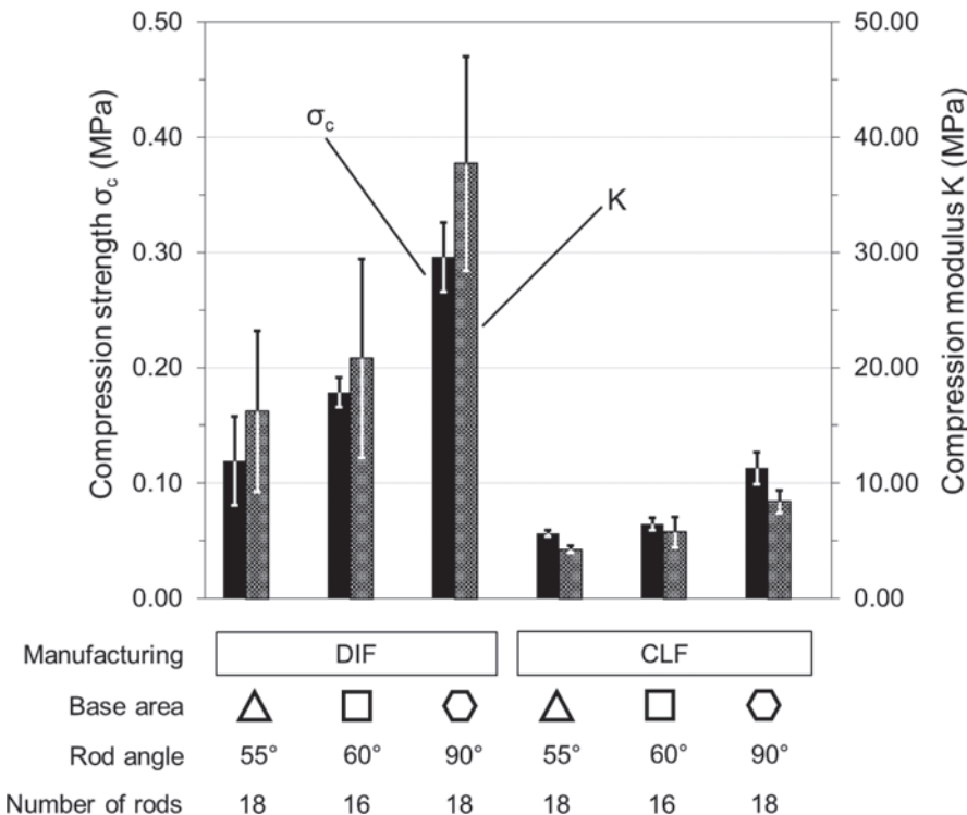
Figure 10: Compression strength \sigma_c and compression modulus K depending on variation for DIF and CLF
