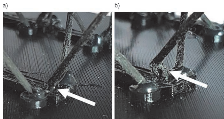
Figure 13: CLF-force transmission, a) before testing, b) after testing
