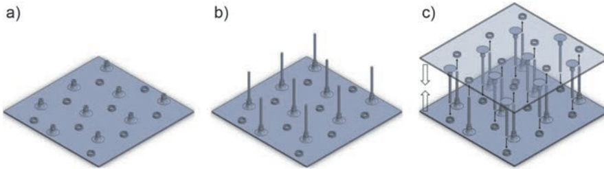
Figure 1: Scheme for differential manufacturing (DIF) process steps, a) individual top layers (FFF), b) manufacturing of lattice core structure, c) manual assembly
