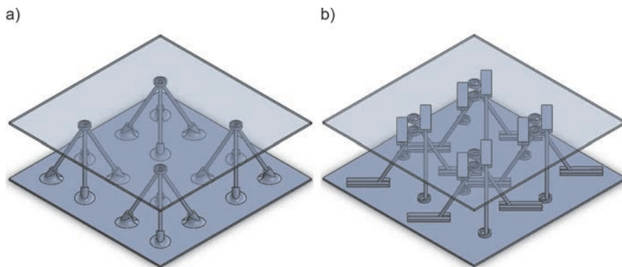
Figure 6: Sandwich panels with a quadratic lattice core structure, a) DIF, b) CLF
